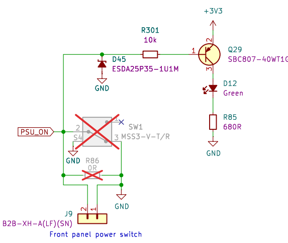
Power switch connector
