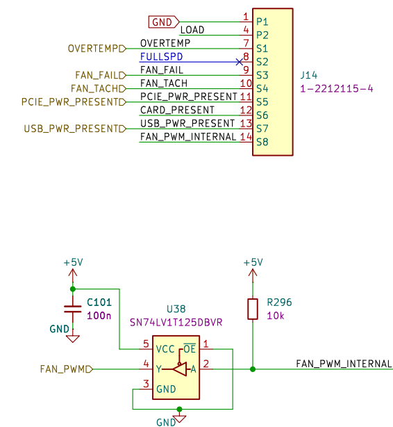
GPU Adapter connector
