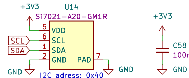
Temperature and humidity sensor
