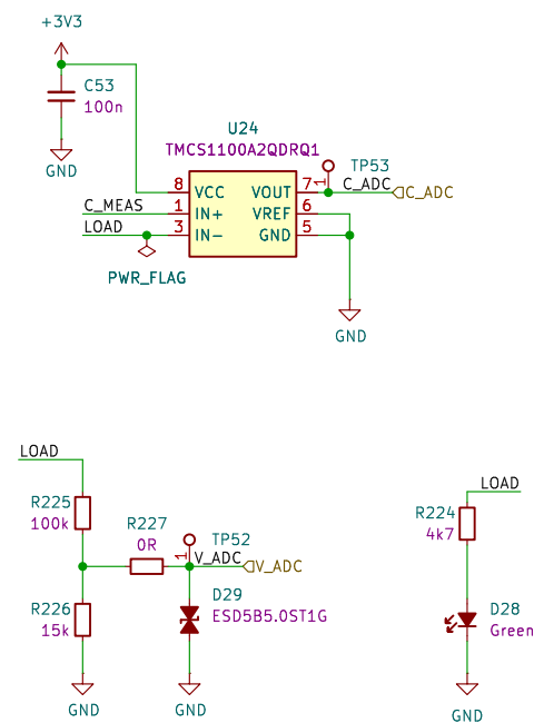
Current and voltage measurement
