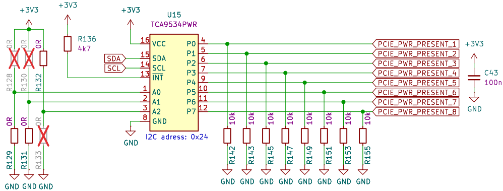
GPIO EXPANDER for PCIE_PWR_PRESENT
