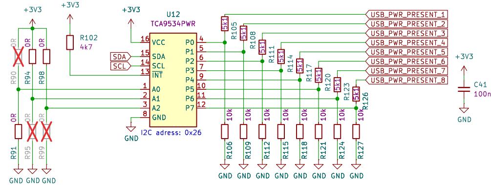
GPIO EXPANDER for USB_PWR_PRESENT
