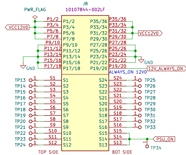
Dell D1600e PSU connector
